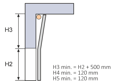
VERTICAL IND-VL
